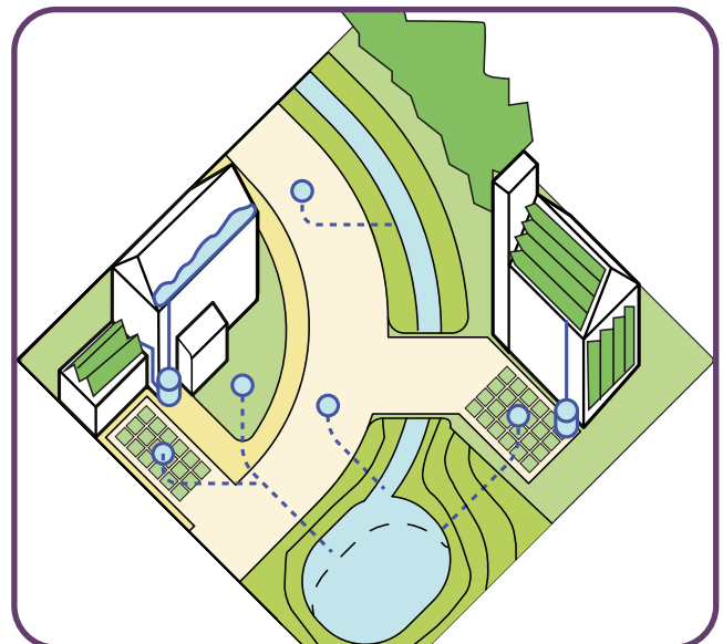
Figure 63: Diagram showing the best use of harvesting water systems rain garden, swales, permeable paving, green roofs..
