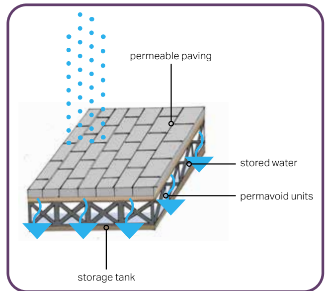
Figure 65: Diagram illustrating the functioning of a soak away.
