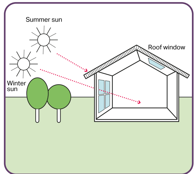
Figure 32: The use of roof window, pitch roof, location and size of windows in favour of maximising solar gain
